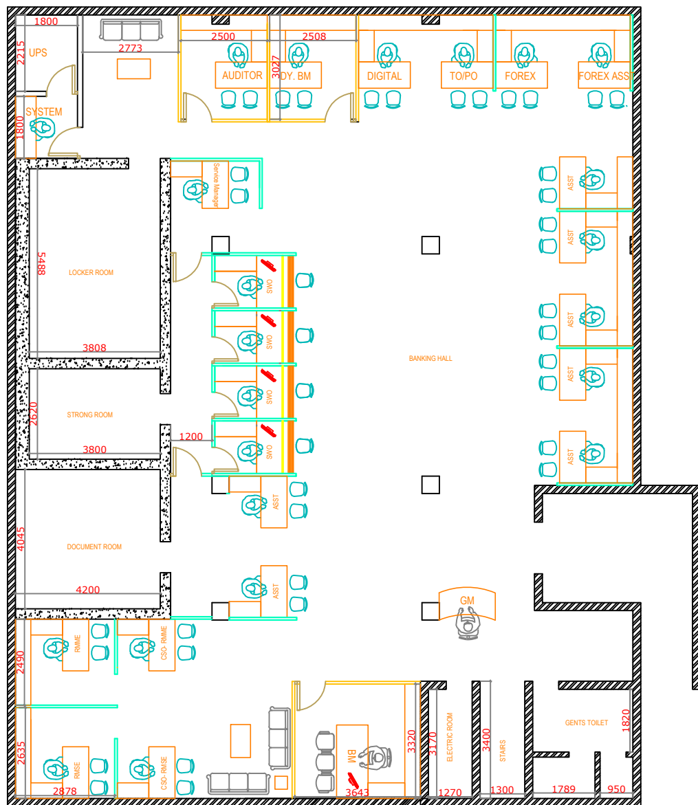
GROUND FLOOR
