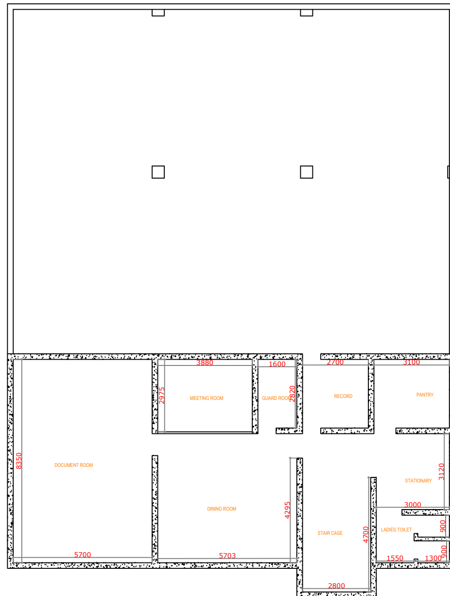
FIRST FLOOR
